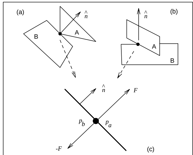
Figure 3. (a) Vertex-plane contact (side view). (b) Edge-edge contact. (c) Contact geometry.
