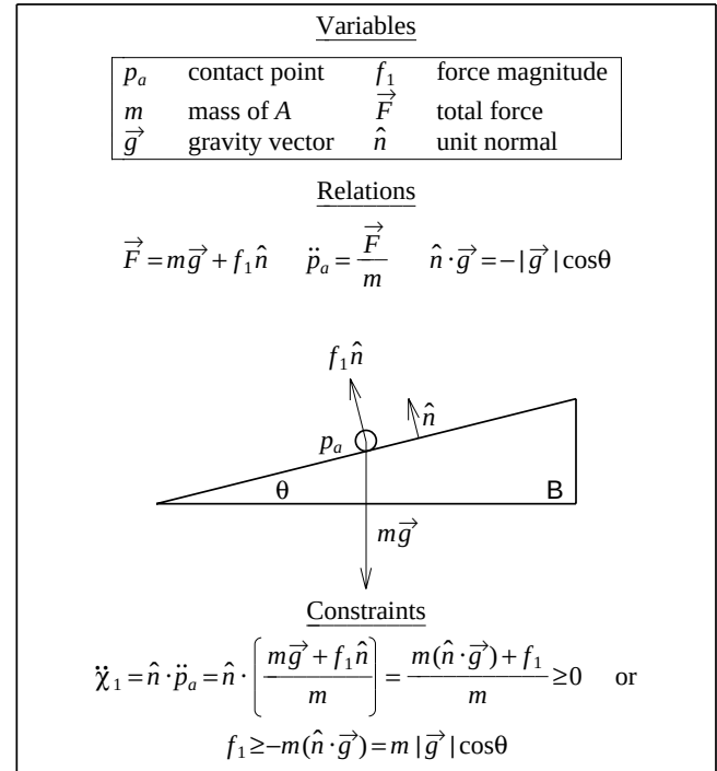
Figure 7. Constraint equations for a point mass A (with position p_a ) resting on a fixed inclined plane B .
