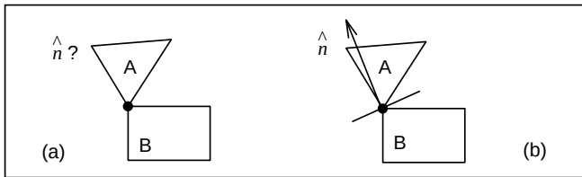
Figure 4. (a) Indeterminate vertex-vertex contact or vertex-edge contact (side view). (b) Removing indeterminacy by choosing \hat{n} .
