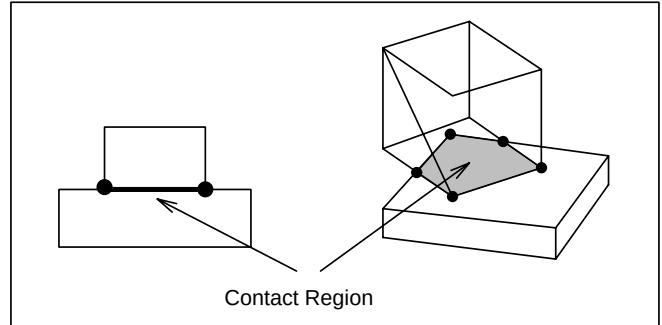
Figure 5. The contact force is assumed to be zero except at points marked with •.
