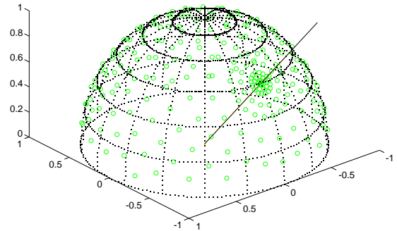
Figure 9: Sampling positions of BRDF measurements on the hemisphere above the sample surface. The solid line indicates the specular reflection direction.
